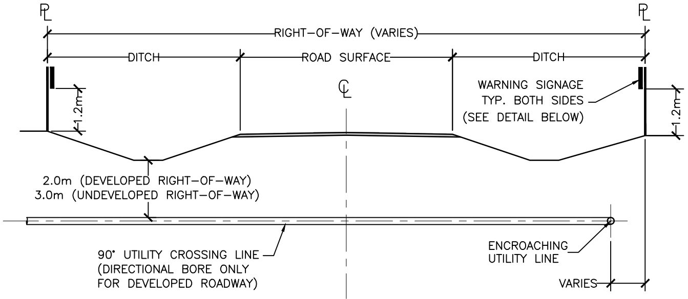
SECTION VIEW
